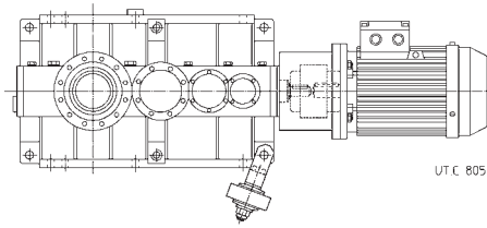
Semi-flexible and economic reaction arrangement (ch. 15): with bolt using disc springs, with bolt and fork using disc springs.
