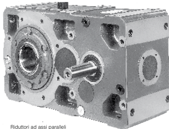
Riduttori ad assi paralleli Parallel shaft gear reducers (2I, 3I 140, 180, 225, 280, 360)
