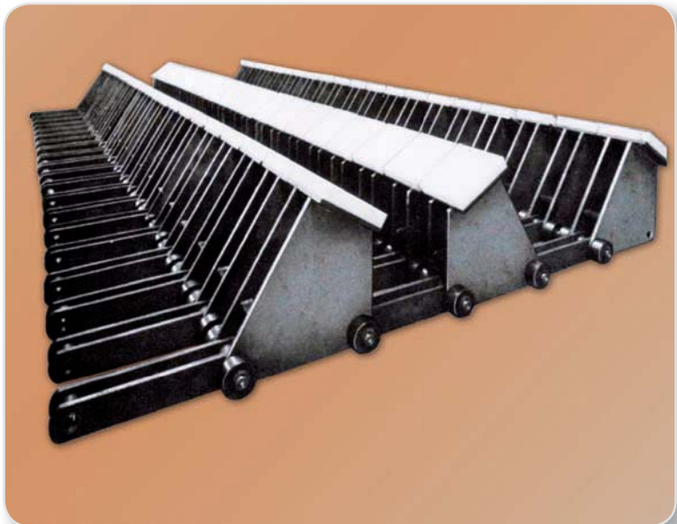
Alumina coil conveyor chain pitch 630 mm with PA supporting.
