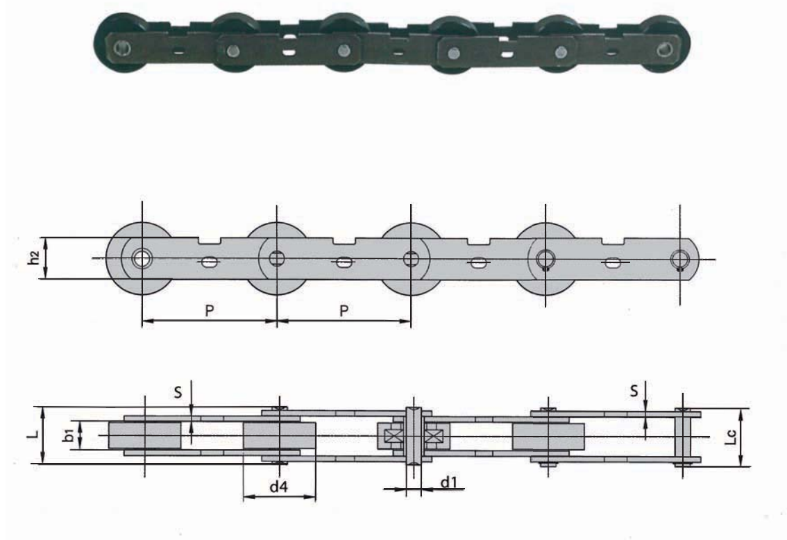
Passenger conveyor chain
