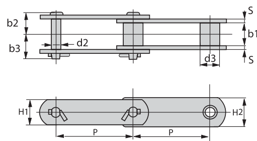
Heavy-duty Z type chain
