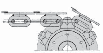
Plate belt conveyor.
