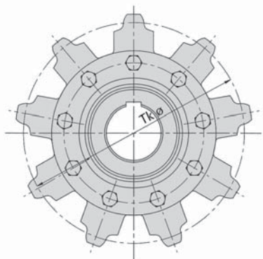
Sizes of chain wheels, pocket teeth, replaceable rims, type GTA
