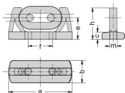
Plug-in attachments SMG
