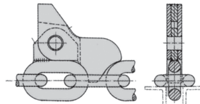
Reversible transport catch.
