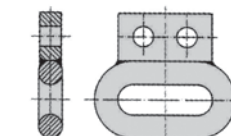
Welded attachment for different transport units.
