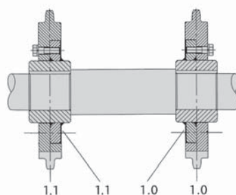
Assembly instruction 2
