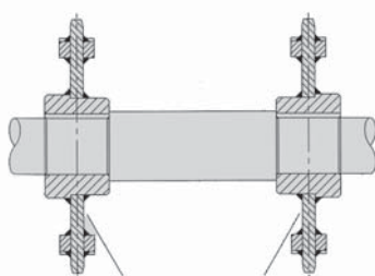
Assembly instruction 1
